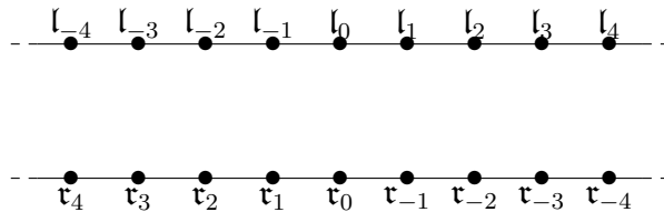
Figure 7.1: An infinite strip with marked points.
